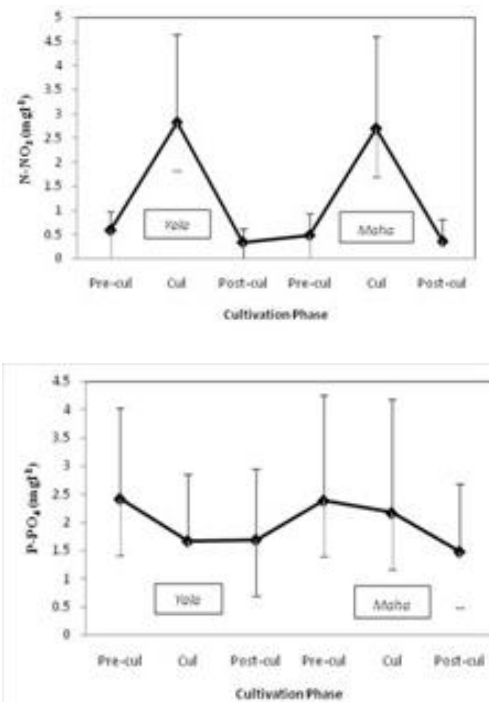
Figure 2: Fluctuation in the mean values of nitrate and phosphate in minor irrigation tanks at pre-cultivation, cultivation and post-cultivation stages of the Yala (n=27) and Maha (n=23) seasons. CEA recommendations for aquatic life nitrate 5 \text{mg l}^{-1} and phosphate 0.4 \text{mg l}^{-1} . Note: although mean values for nitrate are within the safety level, values in some tanks exceed this level as shown in Table 1 and Fig. 3
