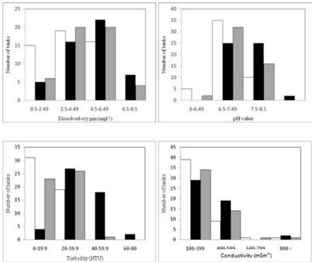
Figure 5. The number of tanks having low to high levels of dissolved oxygen, pH, turbidity and conductivity (mSm -1 ) during pre-cultivation (empty bars), cultivation (black bars) and post-cultivation (grey bars) stages of the paddy cycle.
