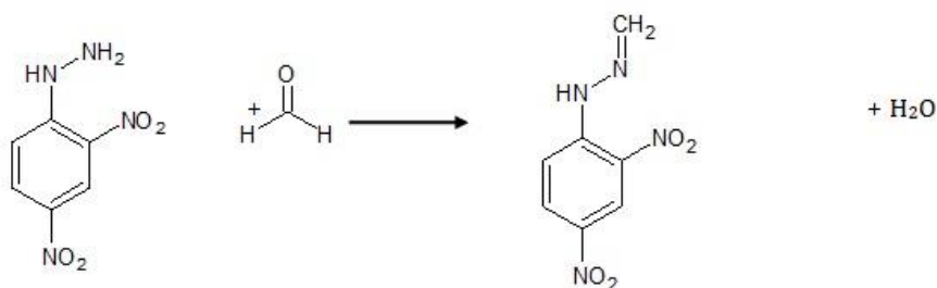
Figure 7. The chemical reaction between formaldehyde and 2,4-DNPH.
