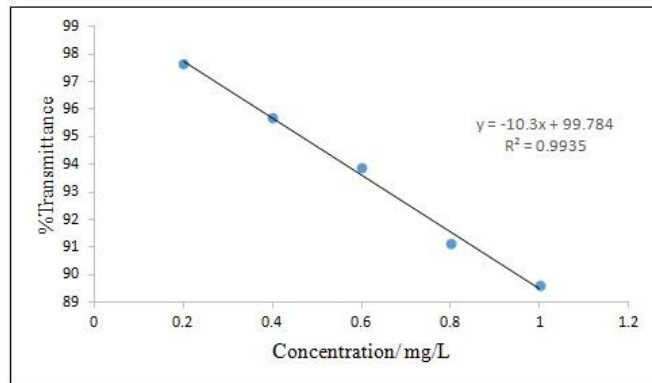
Figure 5. Correlation between the FTIR %transmittance and the formaldehyde concentrations of 0.2, 0.4, 0.6, 0.8, 1 mg/L.
